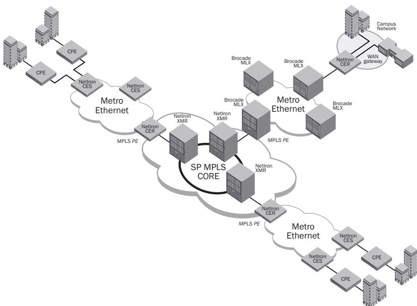
Figure 1: High-performance, secure Brocade solution supports Layer 2 and Layer 3 VPNs.
